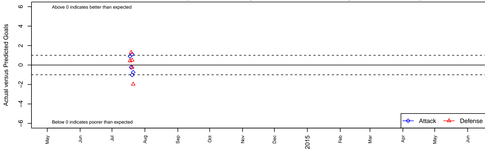
Cook Inlet Velocity 01 Blue G00 Dots are actual minus expected GF (blue circles) and GA (red triangles). Blue line is smoothed change in attack strength. Red is smoothed change in defense strength.
